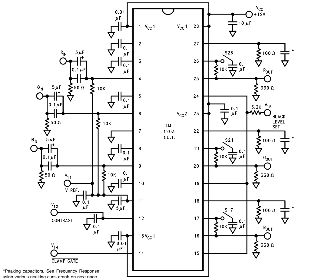
FIGURE 2. LM1203 Test Circuit
